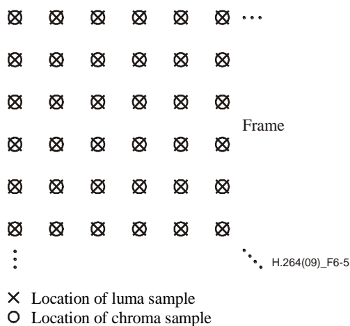
Figure 6-5 – Nominal vertical and horizontal locations of 4:4:4 luma and chroma samples in a frame
