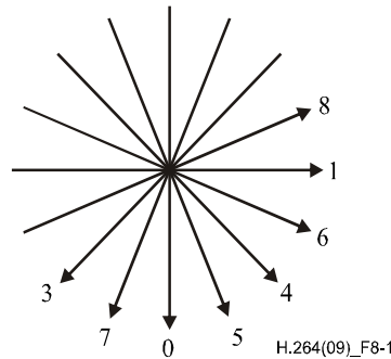
Figure 8-1 – Intra_4x4 prediction mode directions (informative)
