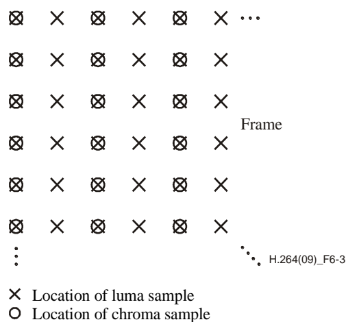
Figure 6-3 – Nominal vertical and horizontal locations of 4:2:2 luma and chroma samples in a frame
